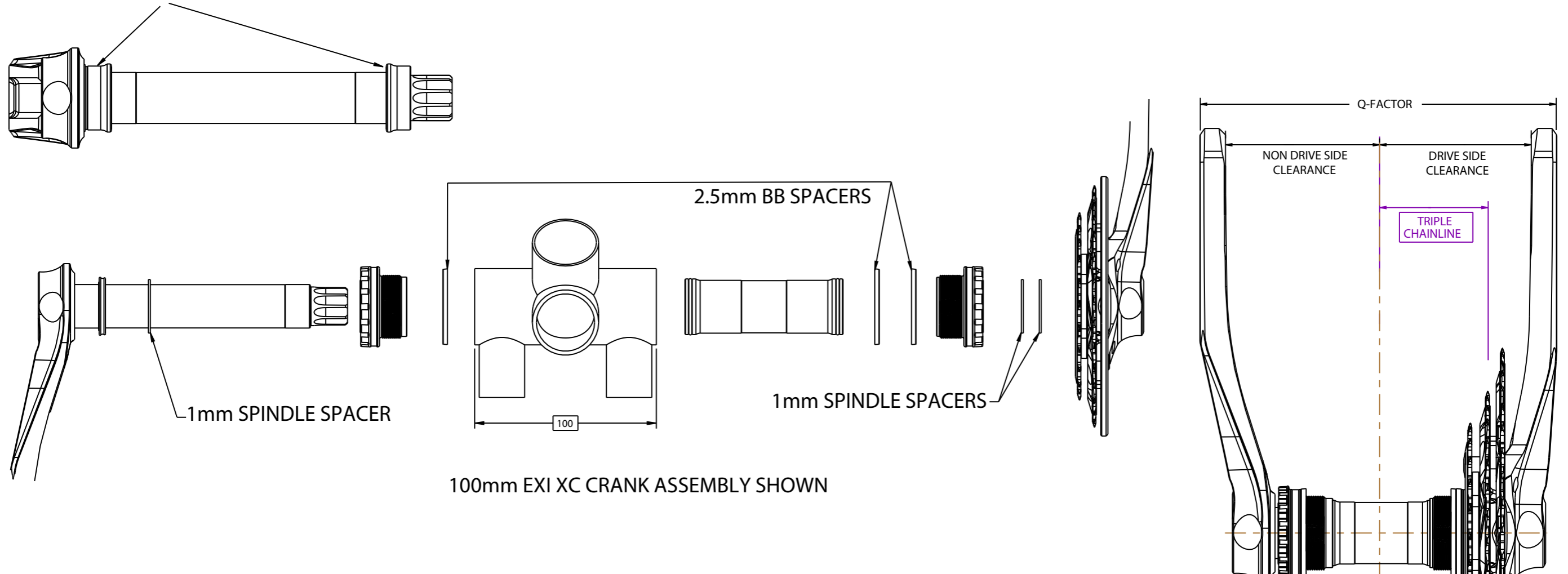
11.5mm SPINDLE SPACERS on 190mm EXI CRANKS
